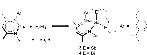
Scheme 2. Chemical equilibrium of 3 and 4 with \text{RGa} and \text{E}_2\text{Et}_4 .
